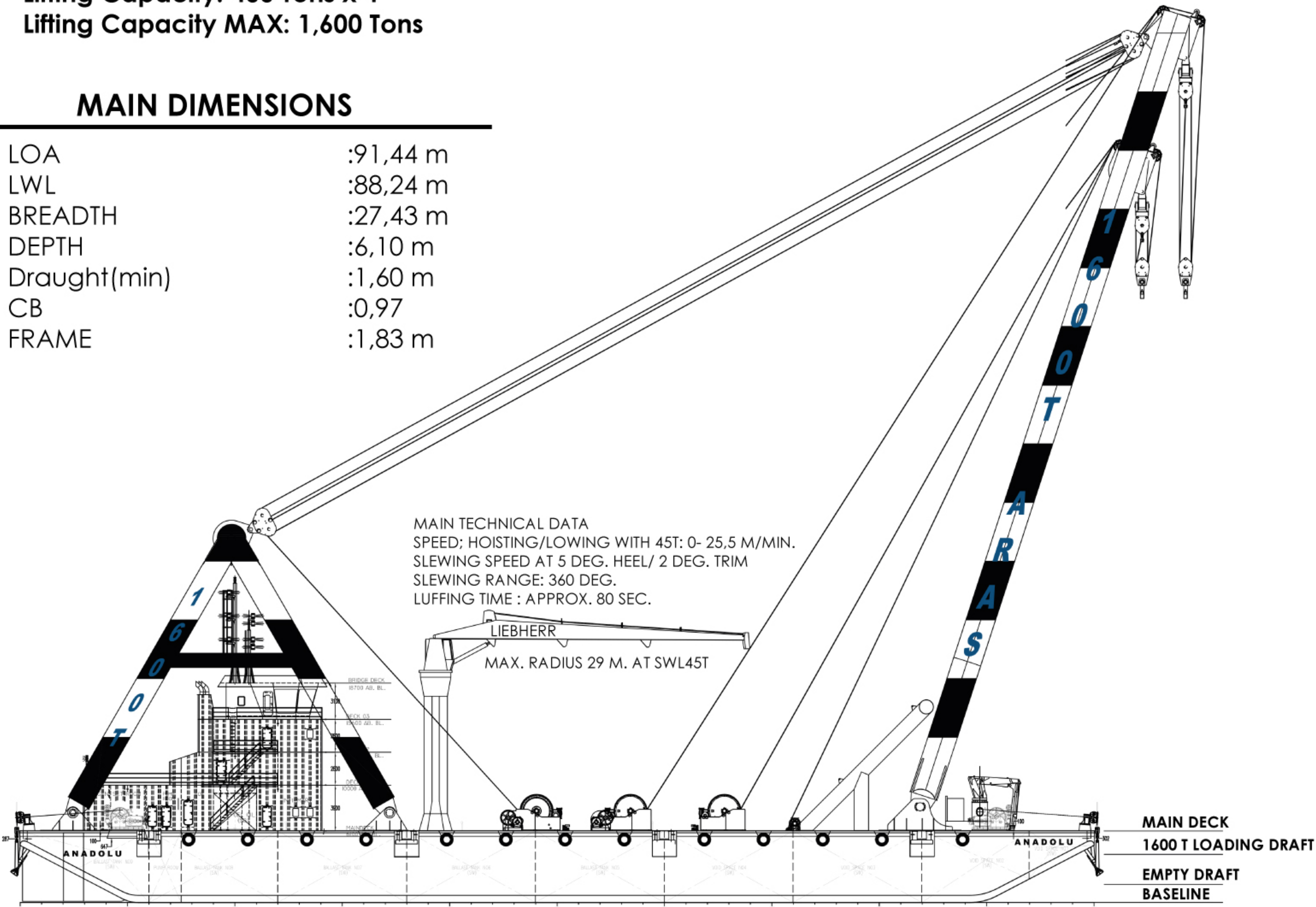
PROFILE VIEW
