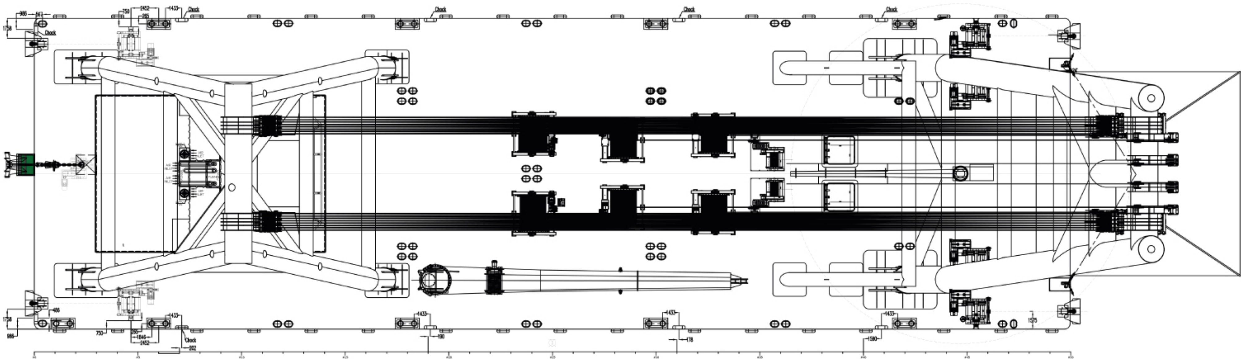
MAIN DECK
